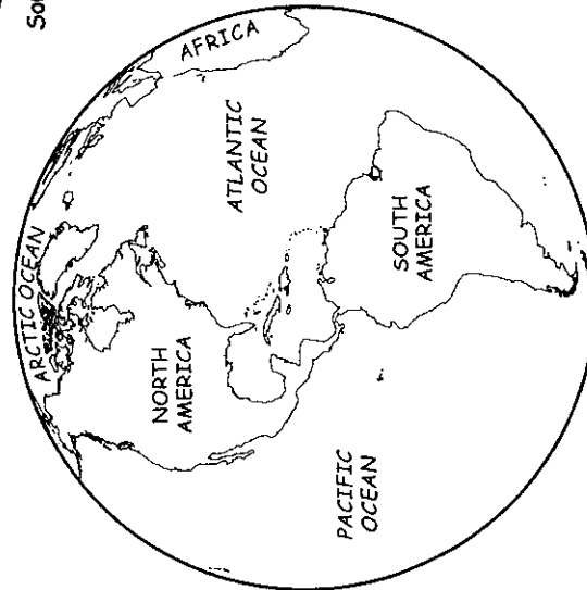
Western Hemisphere
